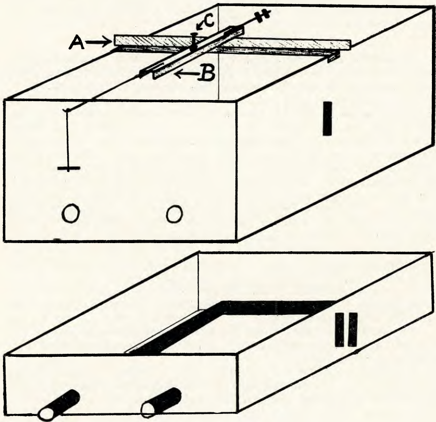
Fig. 35. Incubator unit: Box (I), and Water Pan (II). See text descriptions.
