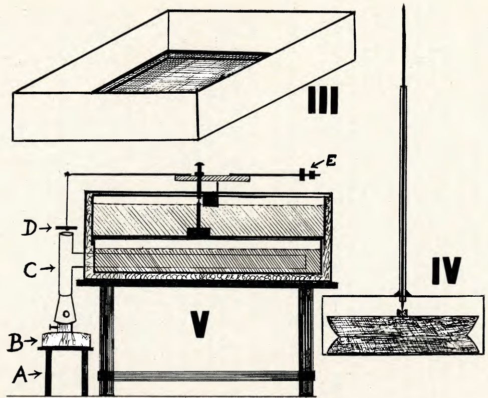
Fig. 36 Incubator unit: Medium Plan (III), thermostat (IV), and complete assembly (V). See text descriptions.
